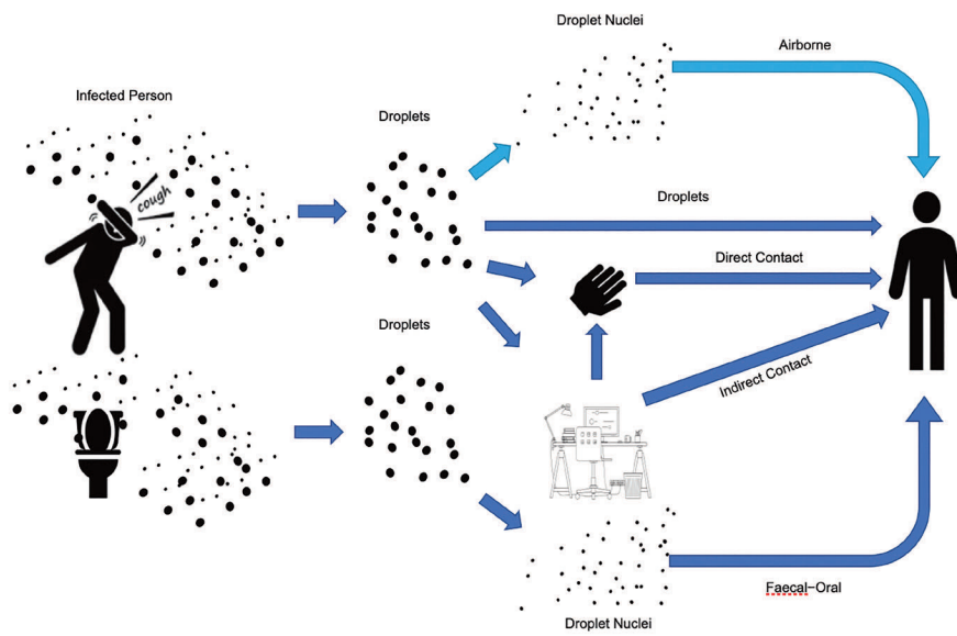
Figure 1. WHO reported exposure mechanisms of COVID-19 SARS-CoV-2 droplets (dark blue color). Light blue color: airborne mechanism that is known from SARS-CoV-1 and other flu, currently there is no reported evidence specifically for SARS-CoV-2 (Figure courtesy of Francesco Franchimon).
